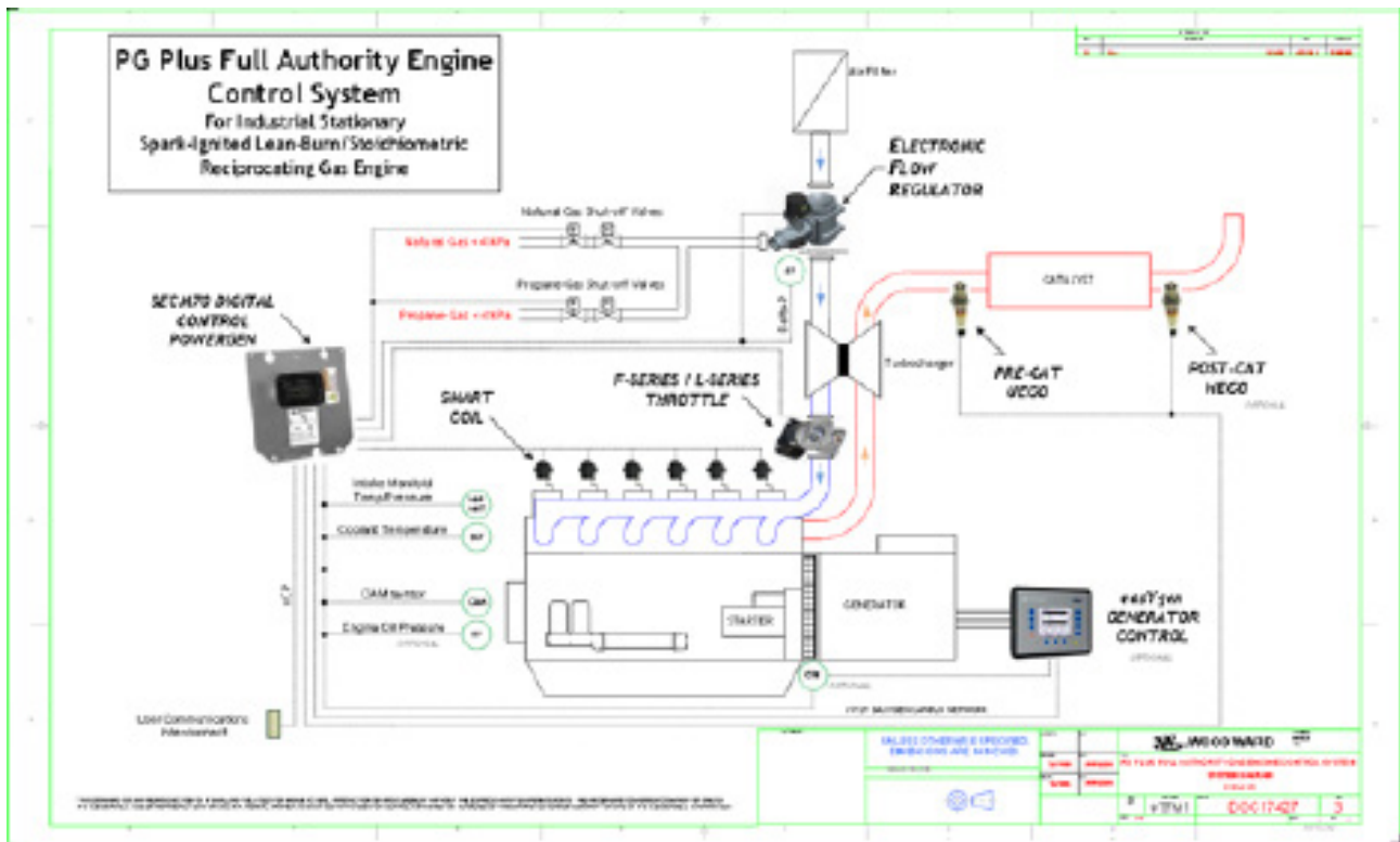
Figure 3. NG/LPG Bi-fuel Engine Control System for Arrow LSI engines
