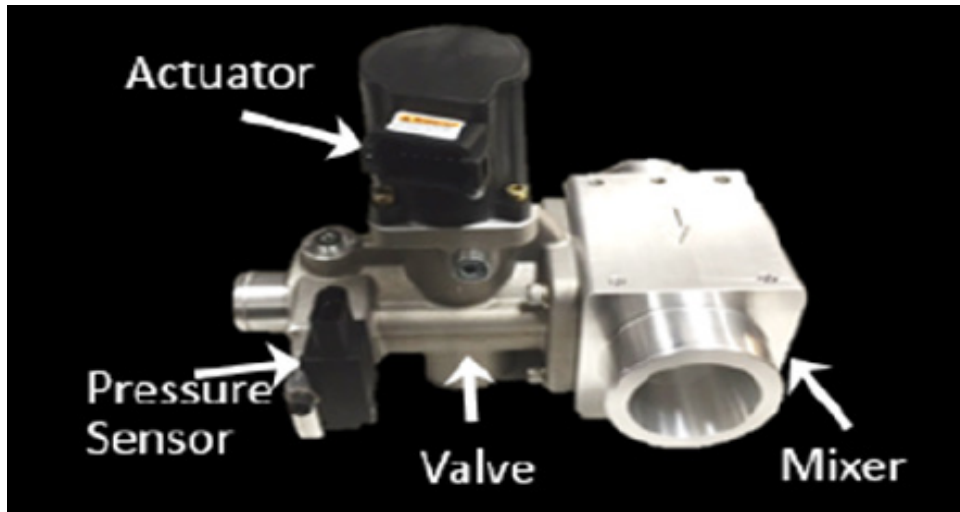
Figure 2. Fuel System Assembly for Arrow LSI engines
